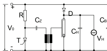
Capacitive triggering with additional booster
