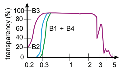
Transparency of borosilicate glasses
