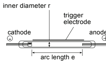
Schematic drawing of a flash tube
