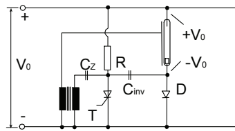
Trigger with doubling of anode voltage
