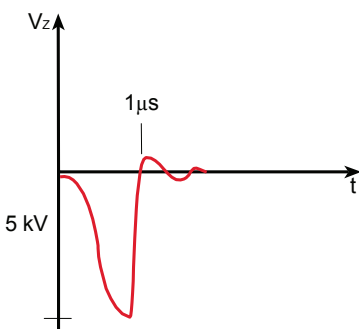
Direct series triggering
