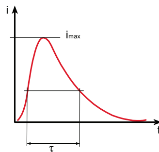
Free capacitor discharge
