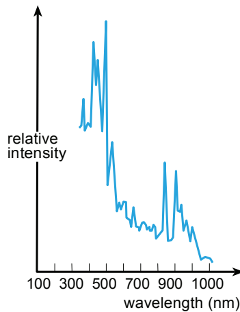
Spectrum of a short arc flashtube
