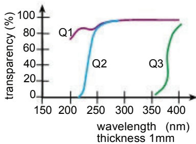
Transparency of quartz glasses
