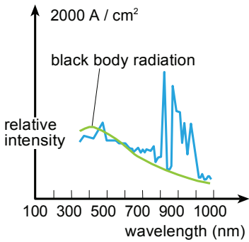
Spectrum of a studio flashtube
