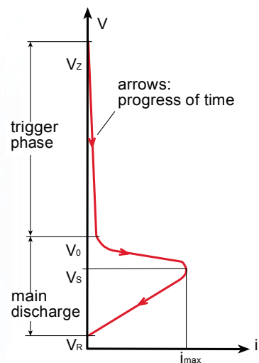
The impedance characteristic of the flash discharge
