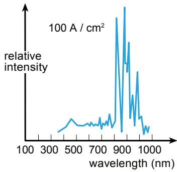
Spectrum of a high impedance flashtube
