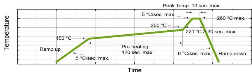
Recommended reflow soldering profile
